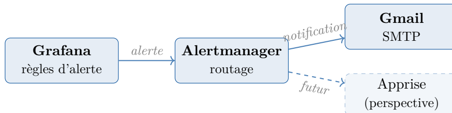
FIGURE III.10 – Pipeline de notification Grafana Alertmanager
